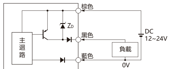
PNP
